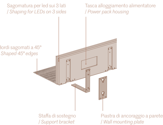
VISTA POSTERIORE / REAR VIEW
